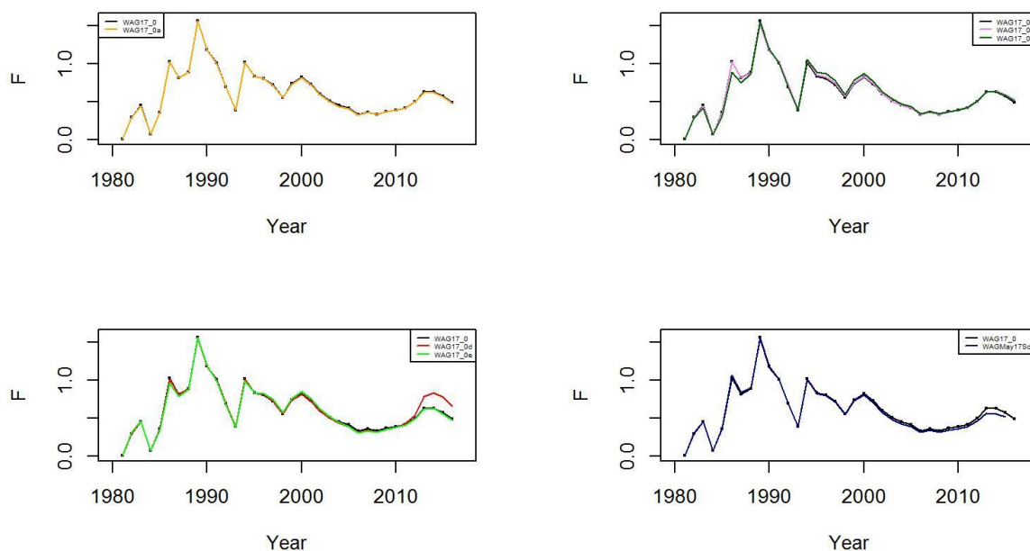
Figure 45. Trends in pot fishery full selection total fishing mortality of golden king crab for scenarios 17_0 to May 2017 Sc9 model fits in the WAG , 1981/82–2016/17.
