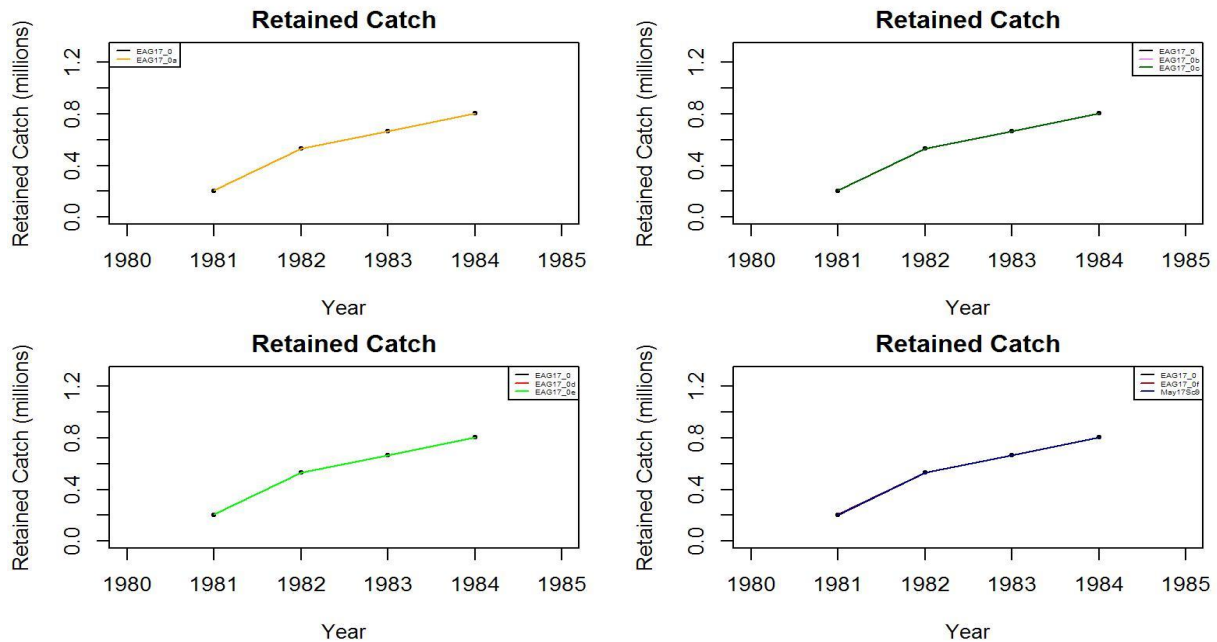
Figure 20. Observed (open circle) vs. predicted (solid line) retained catch of golden king crab for scenarios 17_0 to May 2017 Sc9 fits in the EAG , 1981/82–1984/85. Note: Input retained catches to the model during pre-1985 fishery period were in number of crabs.
