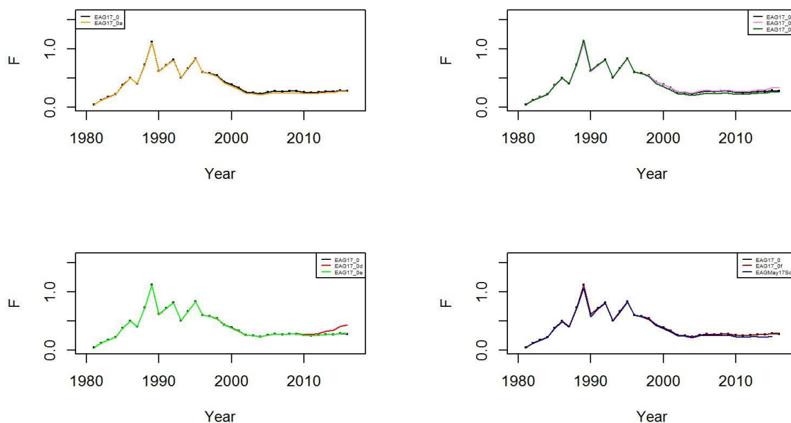
Figure 27. Trends in pot fishery full selection total fishing mortality of golden king crab for scenarios 17_0 to May 2017 Sc9 model fits in the EAG , 1981/82–2016/17.
