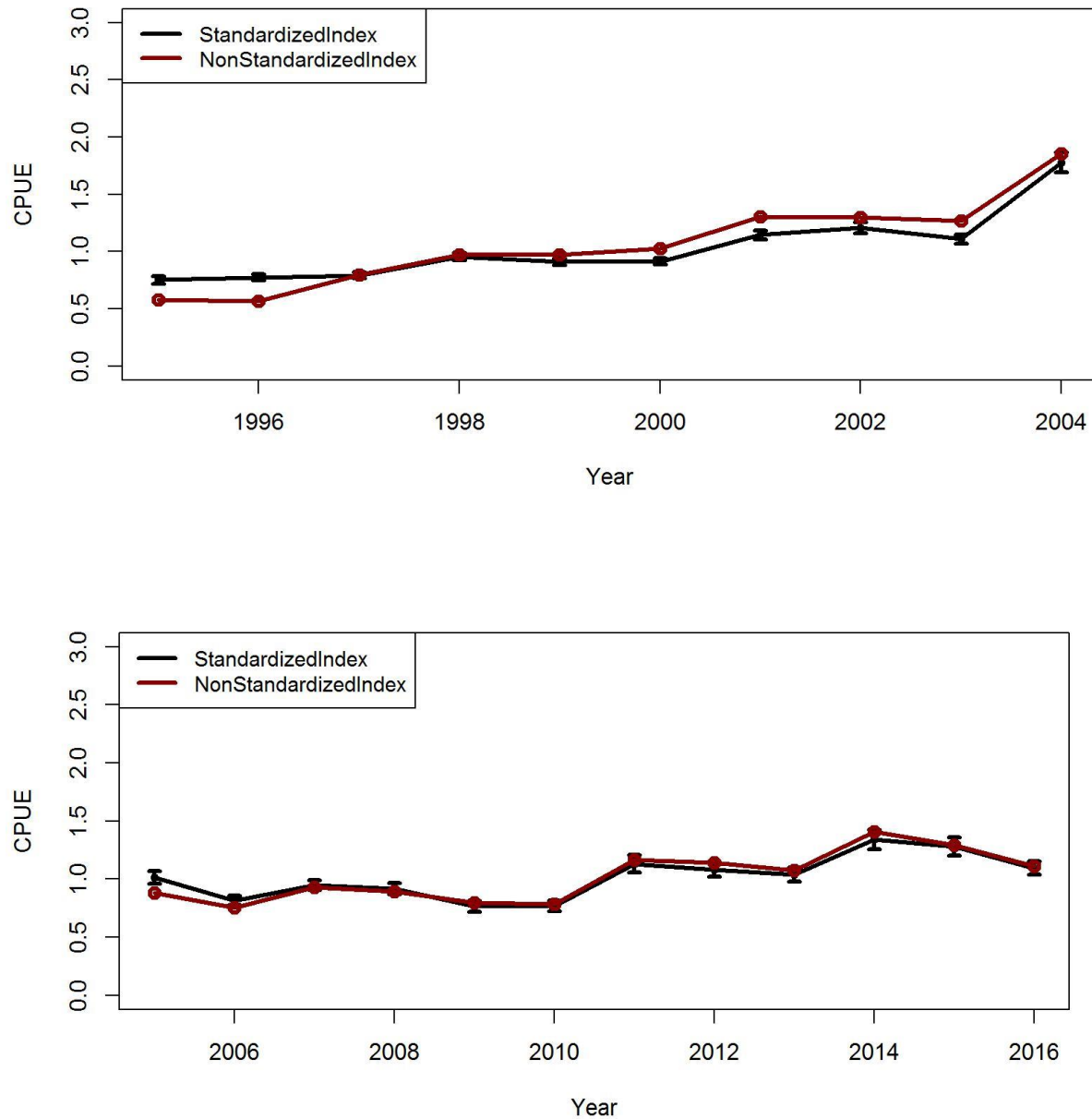
Figure B.1. Trends in non-standardized [arithmetic (nominal)] and standardized (negative binomial GLM) CPUE indices with \pm 2 SE for Aleutian Islands golden king crab observer data from EAG (east of 174^\circ W longitude). Top panel: 1995/96–2004/05, and bottom panel: 2005/06–2016/17. Standardized indices: black line and non-standardized indices: red line. Variable selection by R^2 criteria.
