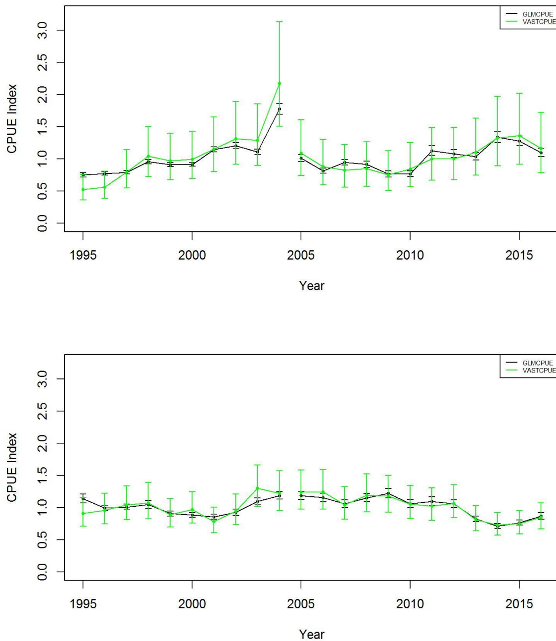
Figure B.7. Comparison of GLM (black) and VAST (green) estimated CPUE indices with \pm 2 SE for Aleutian Islands golden king crab in EAG (top panel) and WAG (bottom panel) for 1995/96–2016/17. GLM variable selection by R^2 criteria.
